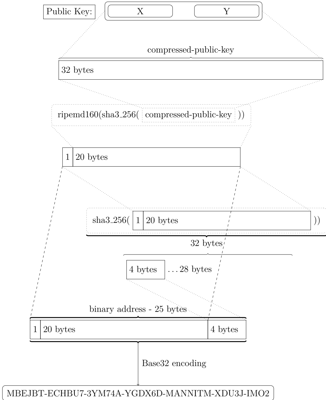
Figure 7: Address generation
