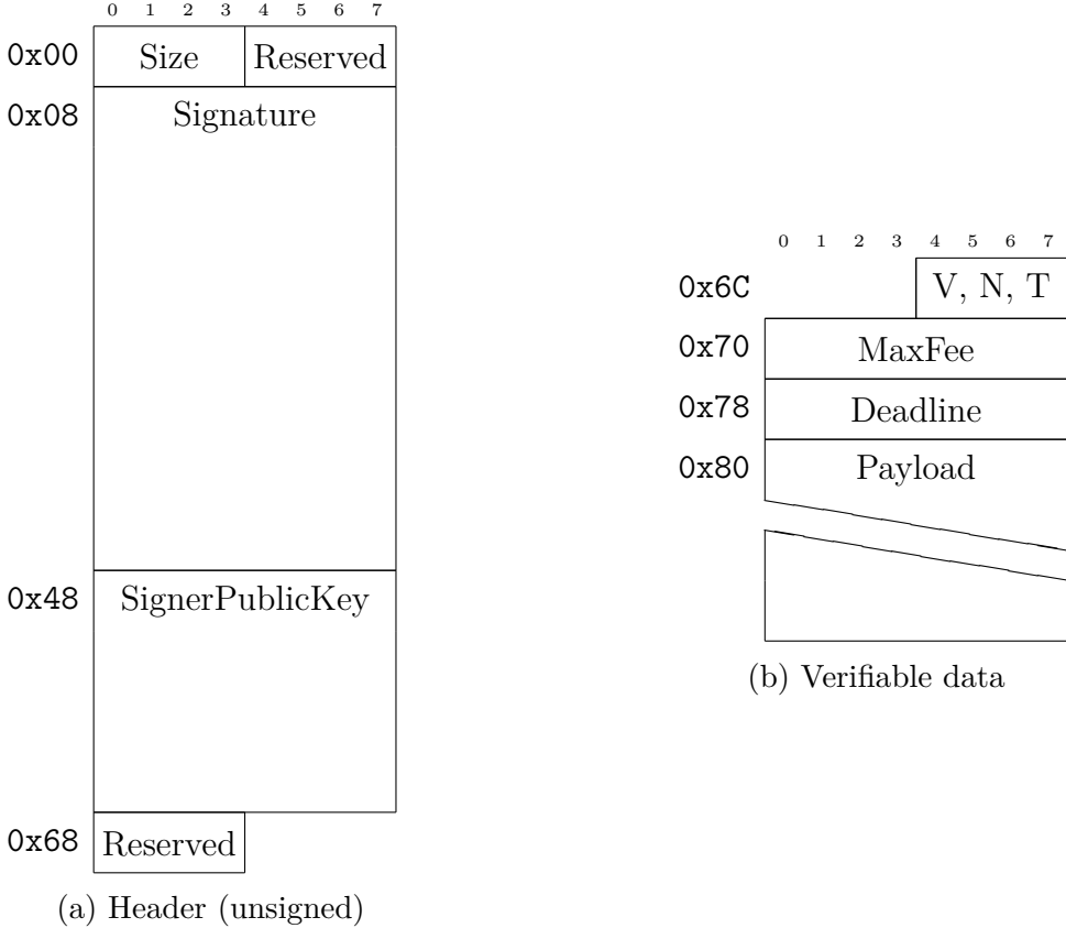
Figure 8: Basic transaction binary layout
