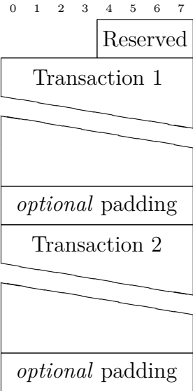
Figure 16: Block transaction footer with padding
