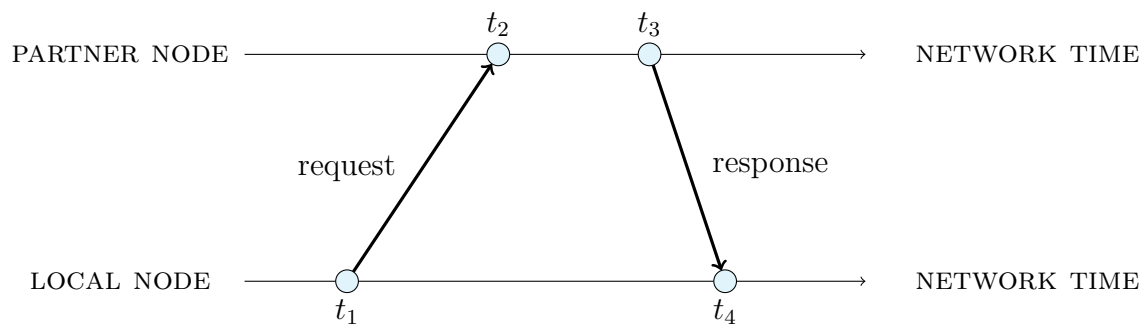
Figure 33: Communication between local and partner node.
