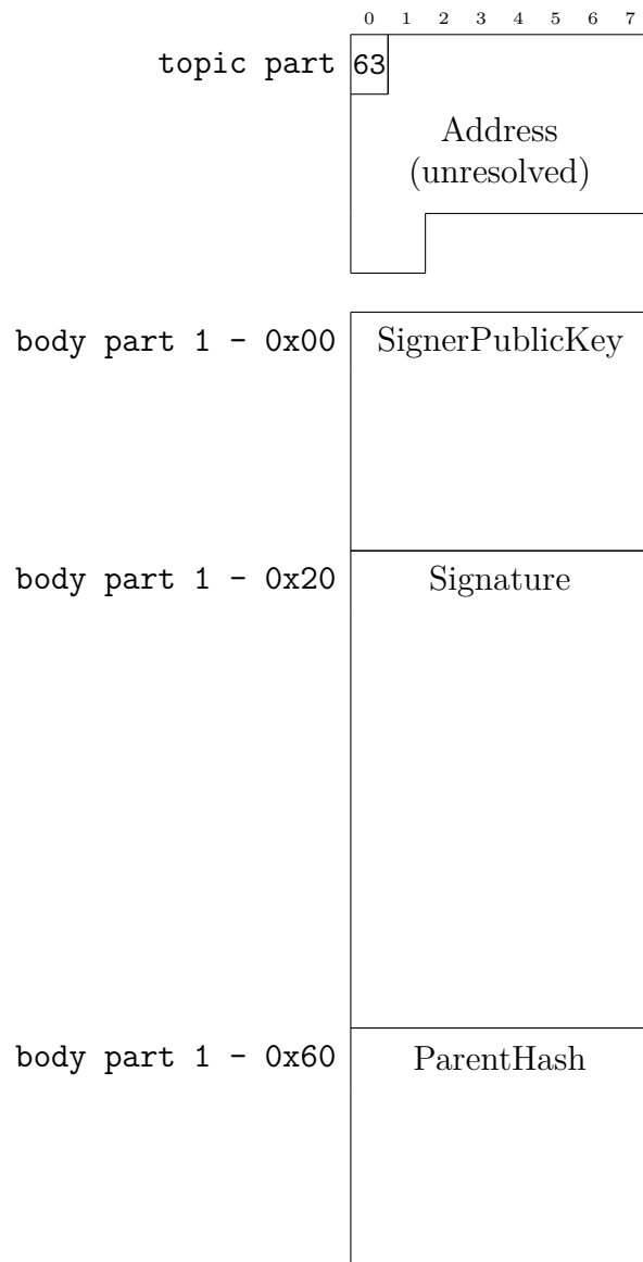
Figure 40: Cosignature message
