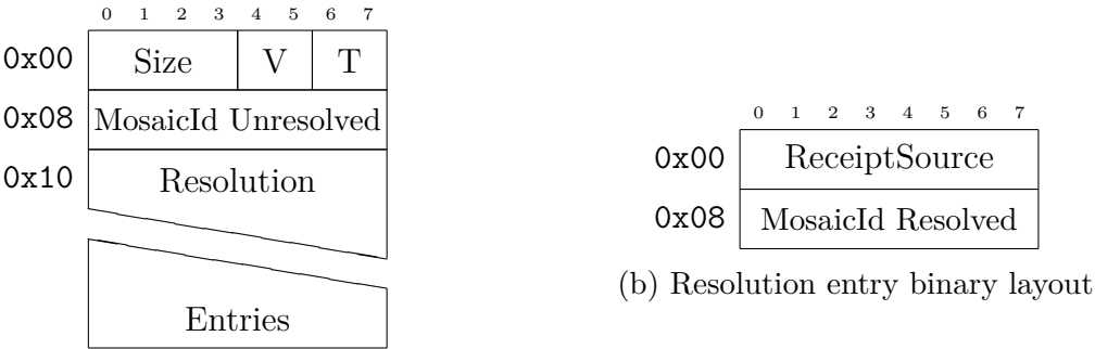
(a) Mosaic resolution statement binary layout
