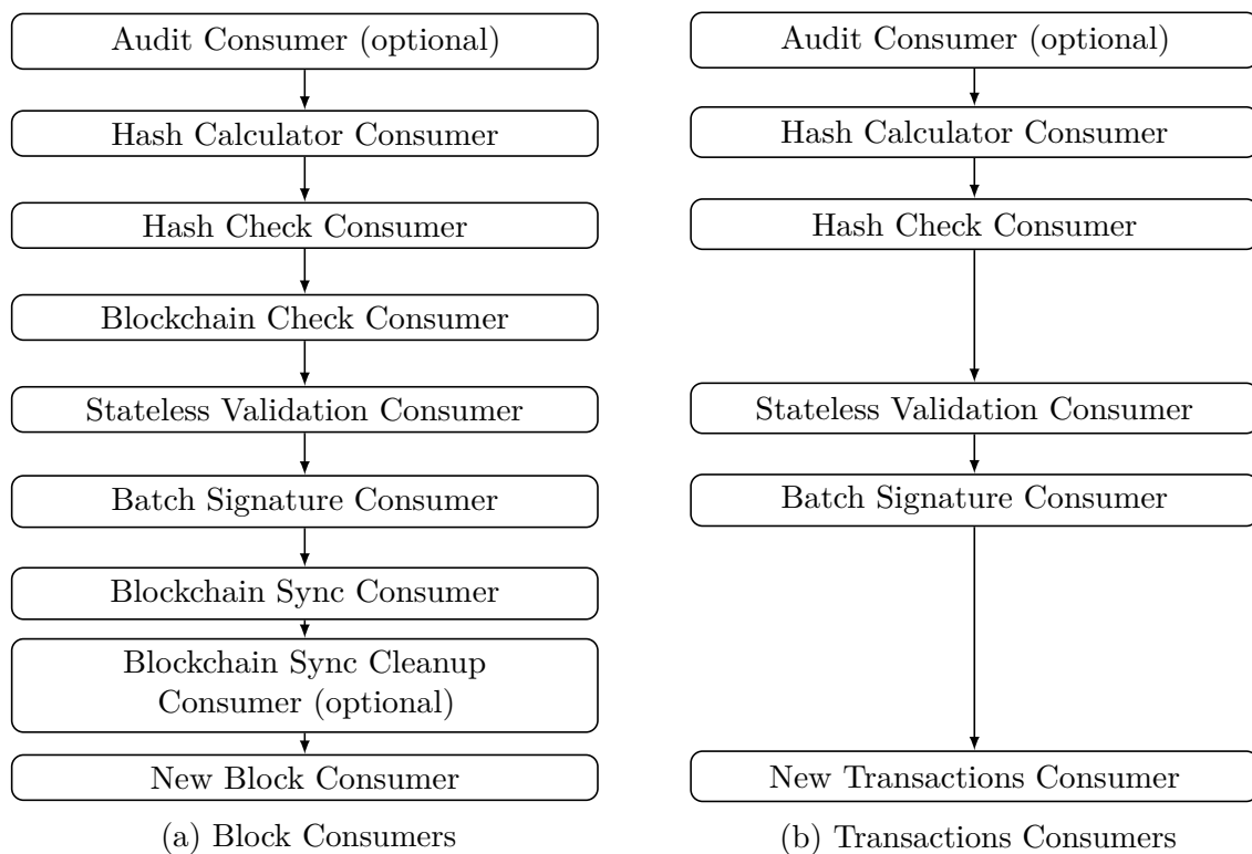
Figure 19: Symbol consumer chains
